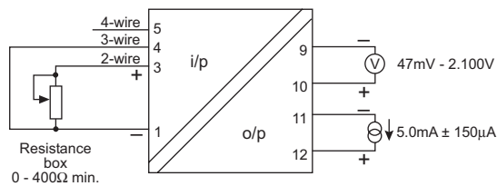
Figure 8.10: AI test circuit #5 "Resistance input"
