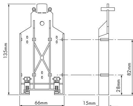
Figure 4.5: IMB57 Insulating mounting block
