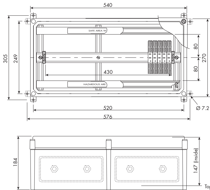
Figure 5.2: DX range of enclosures
