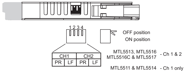
Figure 6.1: Switches to set LFD and phase reversal
