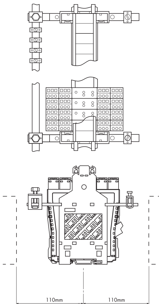
Figure 4.11: MTL5500 complete assembly
