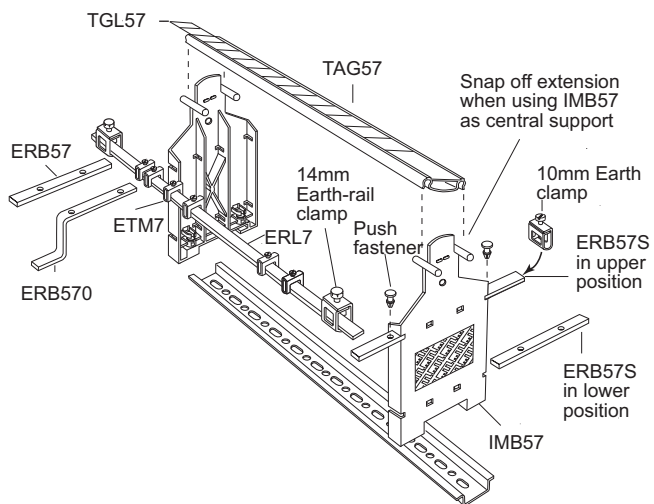
Figure 4.3: Assembly drawing showing part numbers
