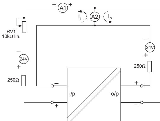
Figure 8.8: AI test circuit #4 "active i/p - o/p sinking"
