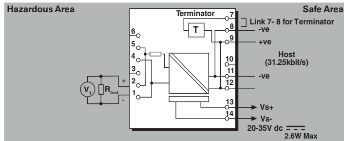
Test circuit for MTL5553
