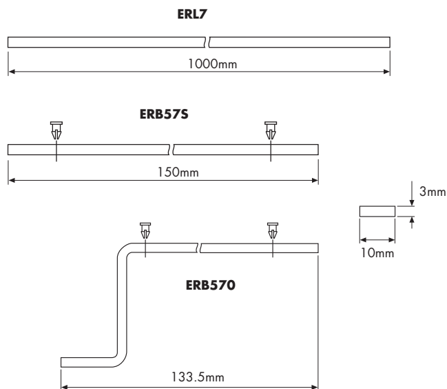
Figure 4.4: Mounting details
