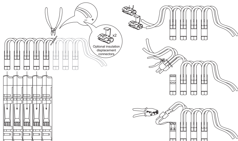
Figure 4.1: Power bus wiring, joining and terminating
