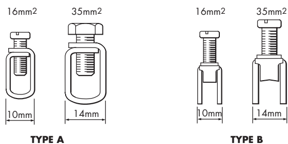
Figure 4.9: Earth rails and clamps
