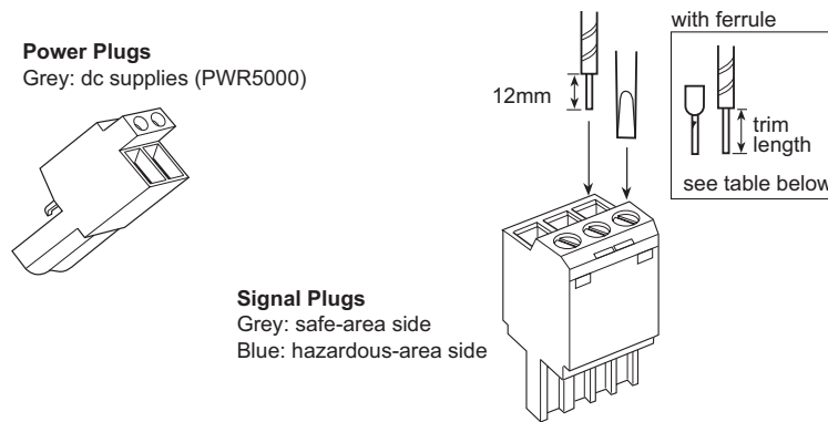
Figure 3.4: Removable power and signal plugs
