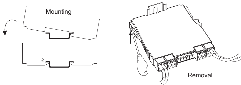
Figure 3.3: DIN rail mounting and removal of isolators
