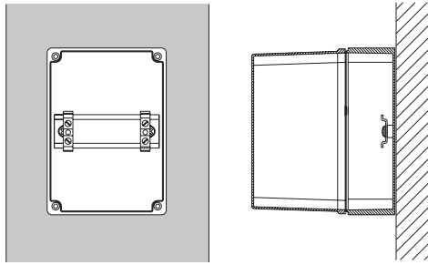
Figure 5.3: Optimum orientation for wall mounted enclosure
