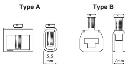
Figure 4.8: ETM7 Earth terminals
