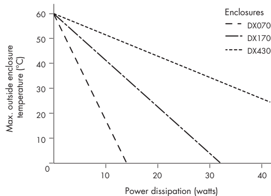
Figure 5.1: Graph depicting outside enclosure temperature limits for DX enclosures used with MTL5500 isolators
