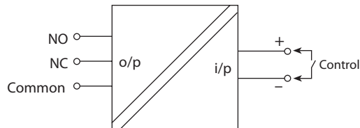
Figure 8.4: DO test circuit for relay type
