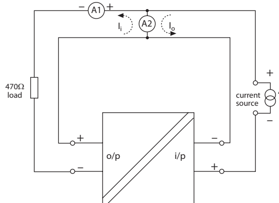
Figure 8.11: AO test circuit
