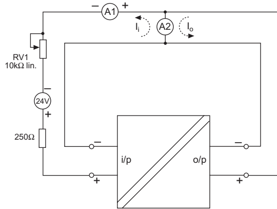
Figure 8.7: AI test circuit #3 "active i/p"
