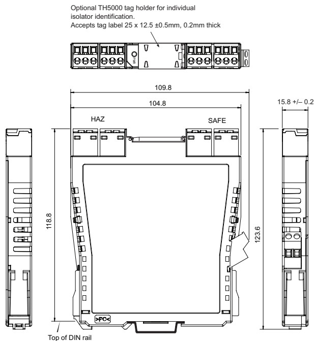
Figure 3.1: Dimensions of MTL5500 package
