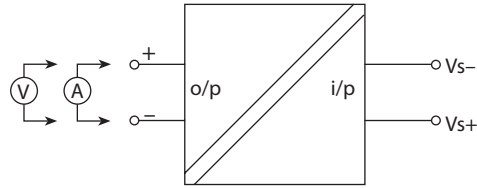
Figure 8.2: Loop powered DO test circuit
