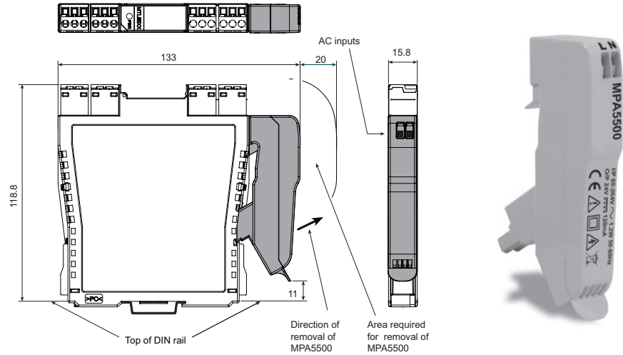
Figure 4.2: MPA5500 AC power adaptor
