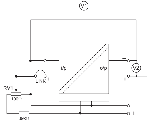
Figure 8.9: AI test circuit #5 "mV input"
