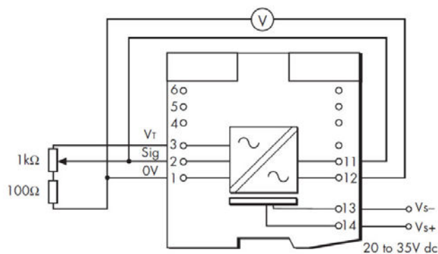
Figure 8.12: Test circuit for MTL5531
