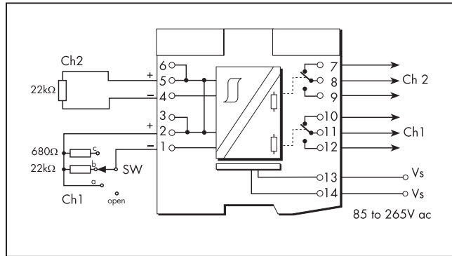
Figure 10.2: Test circuit for MTL5018AC
