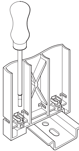
Figure 4.10: Fitting IMB57
